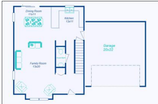
First Floor Option A
